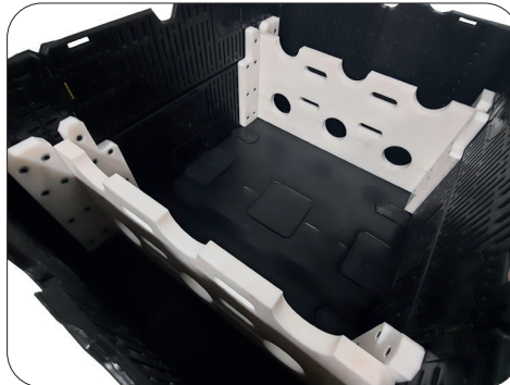
6 Lot MegaPACK İçi Poliamid Separatör / MegaPACK with 6 Lots Polyamid Divider
