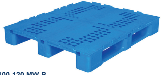
TP-100-120 MW-P Profil Yuvalı / Profile Slot En/W Boy/L Yük/H
