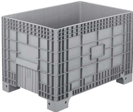
TP-550 En/W Boy/L Yük/H Hacim Dynamic Static Dış / Ext 800 x 1200 x 800 mm Volume Capacity Capacity İç / Int 732 x 1106 x 617 mm 500 Lt 400 Kg 2500 Kg Kapalı / Closed Ağırlık / Weight 22,00 kg
