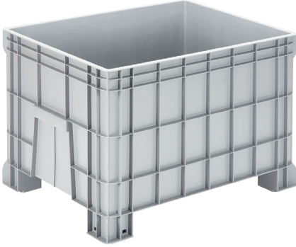
TP-330 En/W Boy/L Yük/H Dış / Ext 670 x 930 x 625 mm İç / Int 620 x 890 x 520 mm
