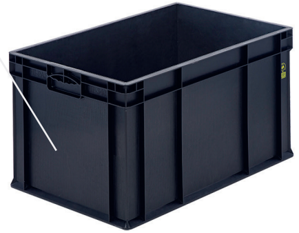
TP-4633 ESD En/W Boy/L Yük/H Dış / Ext 400 x 600 x 340 mm İç / Int 360 x 560 x 324 mm
