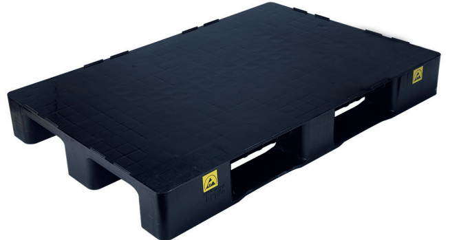
TP-80-120 K ESD En/W Boy/L Yük/H Static Capacity Dynamic Capacity Raf Capacity Dış / Ext 800 x 1200 x 150 mm 3000 Kg 1000 Kg 600 Kg
